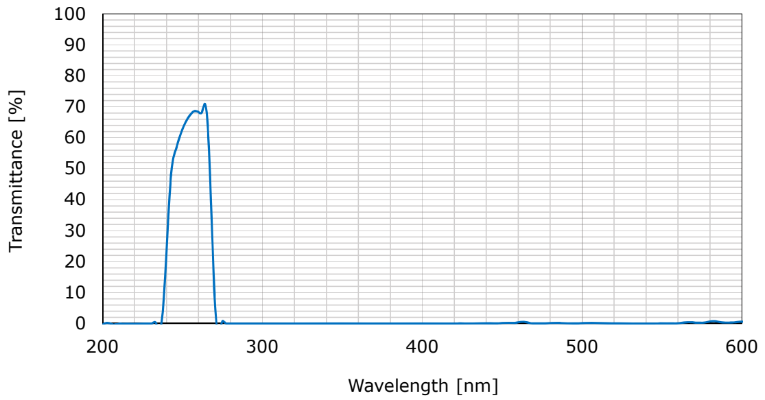
Bandpass filter for UV Sterilization
