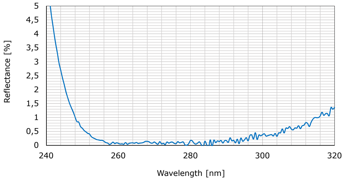
AR Filter for UV Sterilization
